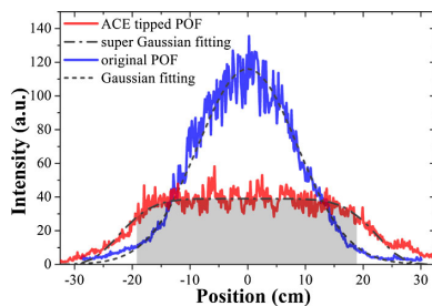
Fig. 4. Measured intensity distributions of the delivered light from an ACE-tipped POF and the original POF counterpart. The grey shadow indicates the ROI for evaluating the degree of inhomogeneity.
