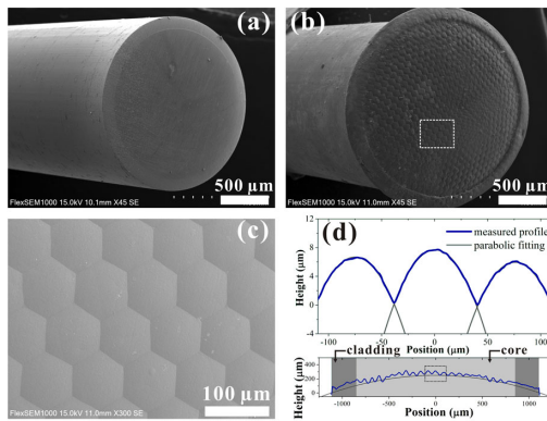
Fig. 1. (a) Polished original planar POF end face. (b) Fabricated ACE-featured POF end face. (c) Zoomed details of the ommatidia [in the dashed box in (b)]. (d) Cross section profile of the ACE end face and the details at the central part (indicated by the dashed box).
