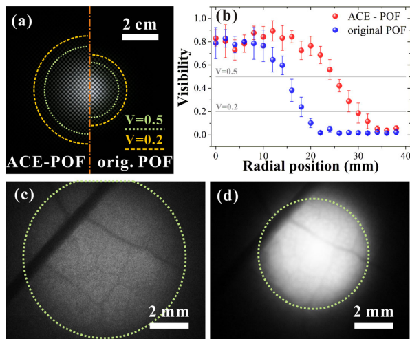
Fig. 5. (a) Checkerboard target illuminated by ACE-tipped POF samples and its original counterpart. (b) Measured visibilities for two illumination conditions. The transmission images of the leaf sample with NIR illumination beam delivered by (c) the ACE-tipped POF and (d) the original POF.
