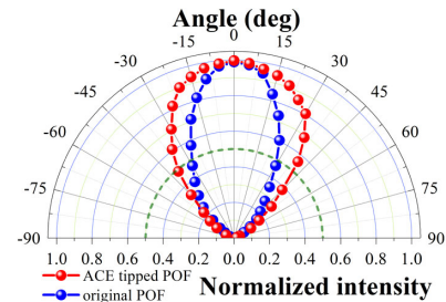
Fig. 3. Normalized angular intensity distributions measured with both an ACE-tipped POF and its original counterpart.
