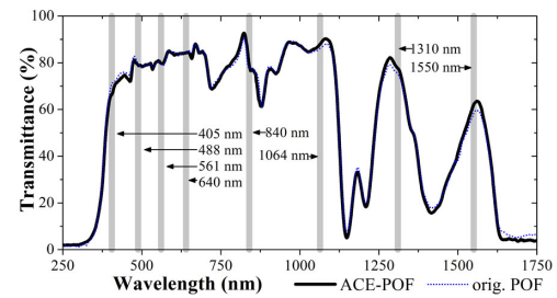
Fig. 2. Transmittances of the fabricated ACE-tipped POF sample and its original counterpart.
